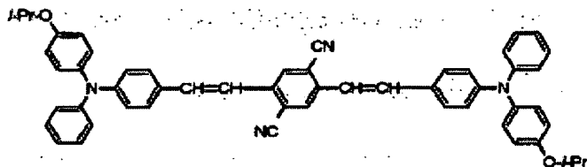
Structural formula (15)-8:
